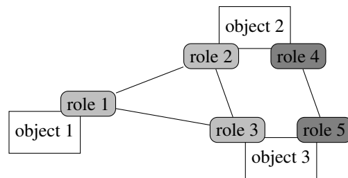
Figure 1: Roles 1 to 3, as well as roles 4 and 5 form two distinct collaborations that can describe independent concerns.
