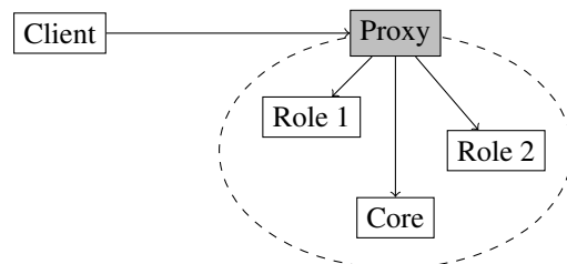
Figure 2: The proxy intercepts calls to the compound object and delegates them via an invocation handler.
